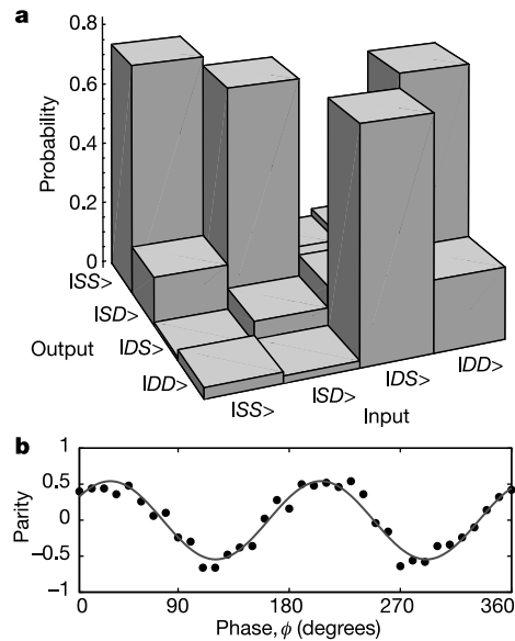
Figure 3 Cirac-Zoller CNOT gate operation. a , Experimentally observed truth table of the Cirac-Zoller CNOT operation derived from joint-probability measurements as in Fig. 2. Ideally, the table should reproduce the squared moduli of the entries of the unitary operation given in equation (1). Experimentally, we find that the currently available fidelity of the gate operation is limited to about 70–80%; detailed values of measured probabilities are listed below:
