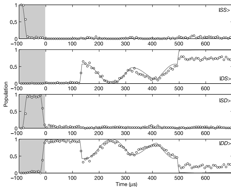
Figure 2 Joint probabilities for the ions prepared in |DD\rangle . The data points represent the probability for the ion string to be in the state indicated on the right-hand side. Shaded
