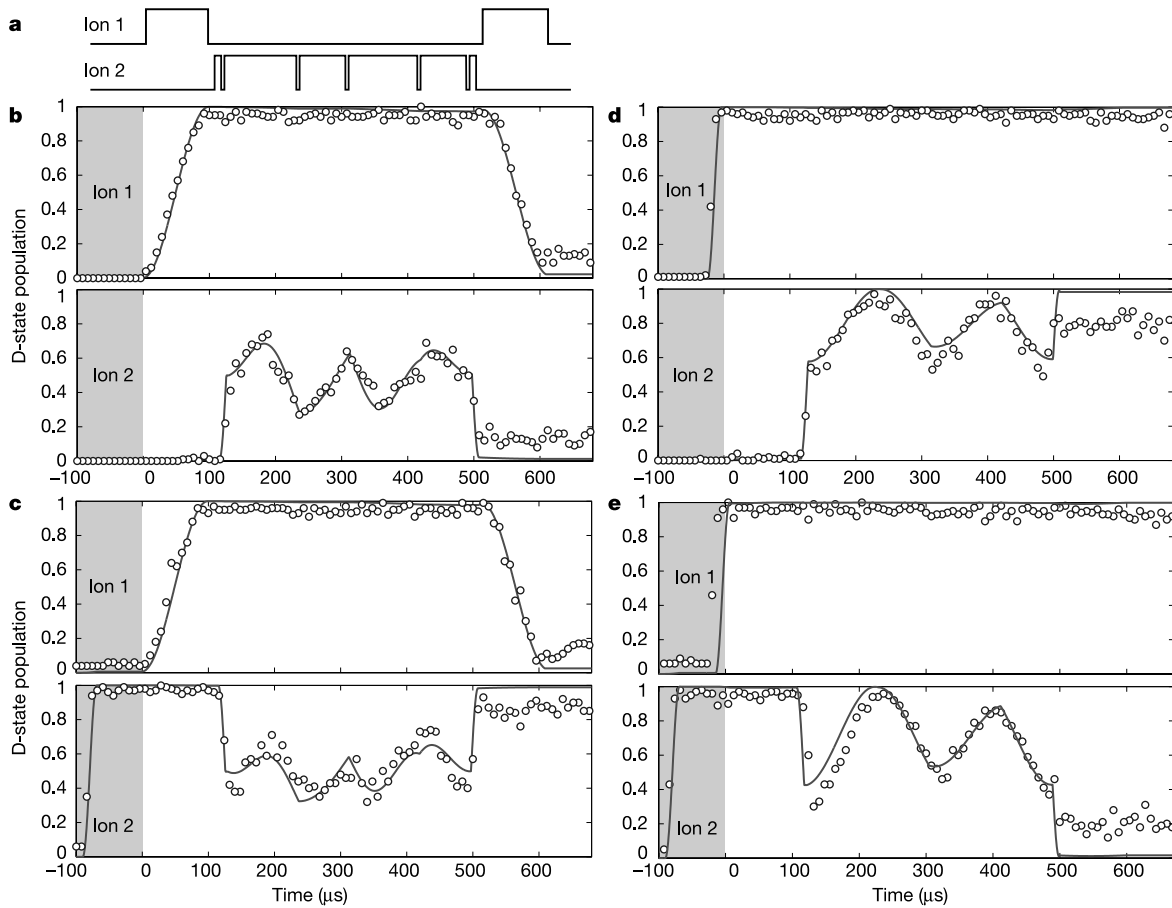
Figure 1 State evolution of both qubits under the CNOT operation. For this, the pulse sequence (a) (see also Table 1) is truncated as a function of time and the D_{5/2} state probability is measured (b–e). The solid lines indicate the theoretically expected behaviour. They do not represent a fit. Input parameters for the calculations are the independently measured Rabi frequencies on the carrier and sideband transitions and the addressing error. The initial state preparation is indicated by the shaded area and drawn in
