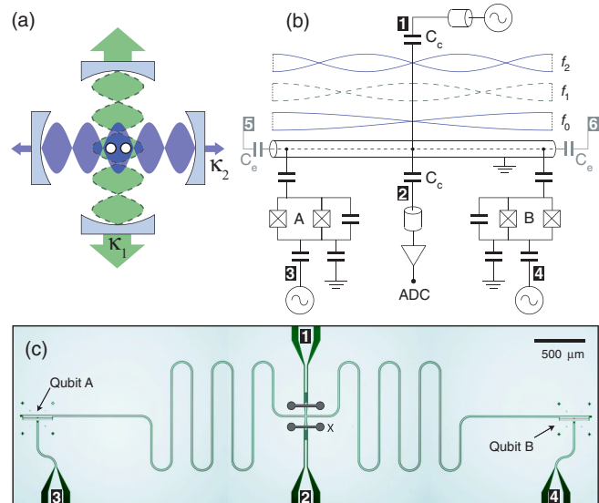
FIG. 1 (color online). (a) Crossed optical Fabry-Perot cavities with two atoms for experiments with two different photon lifetimes. (b) Circuit diagram of center coupled transmission line resonator with qubits ( A , B ) at each end. The resonator is driven through port 1, transmission is measured at port 2. Qubits can be directly driven through ports 3 and 4. Resonator end ports 5 and 6 were included only in a test device without qubits. Also depicted are the field amplitude of the first three resonator modes at frequencies f_{0,1,2} . (c) Optical image (colorized) of the device, with two transmon qubits. Grounding bond wires are shown schematically at position X .
