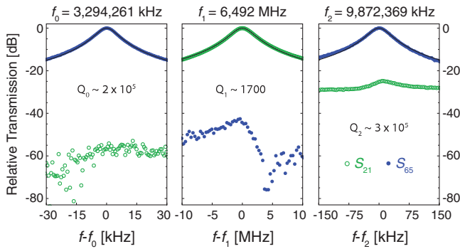
FIG. 2 (color online). Normalized transmission spectrum for a four-port center and end-coupled resonator (device I). Transmission between the end ports S_{65} (blue, closed circles) and the center ports S_{21} (green, open circles) at the fundamental (a), 1st (b) and 2nd harmonic (c) are shown.
