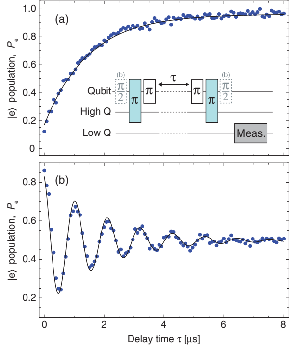
FIG. 4 (color online). (a) Measurement of the lifetime of a single photon in the high Q mode, T_1^{\kappa^2} = 1.45 \mu\text{s} . Inset: Pulse scheme for the experiment with sideband pulses shaded in blue. (b) Results of a Ramsey experiment to measure the photon dephasing time T_2^{*\kappa^2} = 1.9 \mu\text{s} . The pulse sequence is shown in the inset of (a) and described further in the text. Master equation simulations are shown as solid lines.
