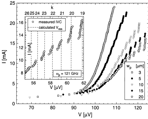
Fig. 1. Current-voltage characteristics of vortex-antivortex state in junctions of different w_p . The calculated resonance voltages and the IVC for w_p = 20 \mu\text{m} are compared in the inset; the voltages are normalized by the number of moving vortices. The top axis indicates the angular wave number of the excited mode.
