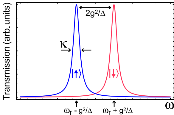
FIG. 5: (color online). Transmission spectrum of the cavity, which is “pulled” by an amount \pm g^2/\Delta = 2.5 \times 10^{-4} \times \omega_r , depending on the state of the qubit (red for the excited state, blue for the ground state). To perform a measurement of the qubit, a pulse of microwave photons, at a probe frequency \omega_{\mu w} = \omega_r or \omega_r \pm g^2/\Delta is sent through the cavity. Additional peaks near \Omega corresponding to qubit flips are suppressed by g/\Delta .
