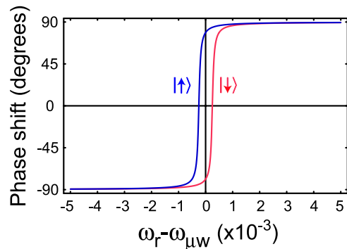
FIG. 8: (color online). Phase shift of the cavity field for the two states of the qubit as a function of detuning between the driving and resonator frequencies. Obtained from the steady-state solution of the equation of motion for a(t) while only taking into account damping on the cavity and using the parameters of Table I. Read-out of the qubit is realized at, or close to, zero detuning between the drive and resonator frequencies where the dependence of the phase shift on the qubit state is largest. Coherent manipulations of the qubit are realized close to the qubit frequency which is 10% detuned from the cavity (not shown on this scale). At such large detunings, there is little dependence of the phase shift on the qubit's state.
