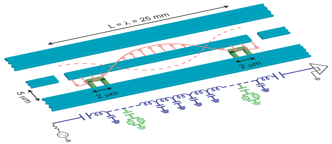
FIG. 1: (Color online) Layout and lumped element version of circuit QED. Two superconducting charge qubit (green) are fabricated inside the superconducting 1D transmission line resonator (blue).
