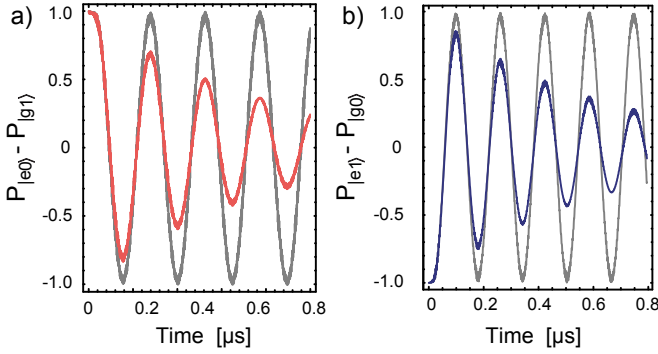
FIG. 7: (Color online) (a) Red and (b) blue coherent sideband oscillations. The system parameters are \omega_a/2\pi = 7 GHz, \omega_r/2\pi = 5 GHz, g/2\pi = 100 MHz. For the color curves, the damping is \kappa/2\pi = 0.22 MHz, \gamma_1/2\pi = 0.02 MHz and \gamma_\phi/2\pi = 0.31 MHz. These last two values are taken from the measured value reported in Ref. [3]. For the gray curves, damping was set to zero. The value of the drive frequencies and amplitudes are: a) \omega_{d_1}/2\pi = 4593.59 MHz, \omega_{d_2}/2\pi = 6650.605 MHz, \varepsilon_1/2\pi = 841.91 MHz and \varepsilon_2/2\pi = 843.417 MHz, b) \omega_{d_1}/2\pi = 4598.39 MHz, \omega_{d_2}/2\pi = 7476.47 MHz, \varepsilon_1/2\pi = 1241.51 MHz and \varepsilon_2/2\pi = 1252.56 MHz.
