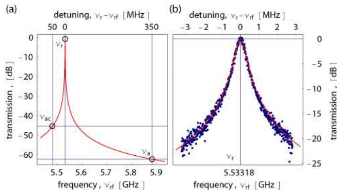
FIG. 2: (color online) (a) Calculated lorentzian cavity transmission spectrum over large frequency range. The cavity drives at frequencies \nu_s \approx \nu_a , \nu_r \approx \nu_r and \nu_{rf} \approx \nu_r and the cavity transmission at these frequencies are indicated. (b) Measured cavity spectrum (dots) and fit (line) around cavity frequency.
