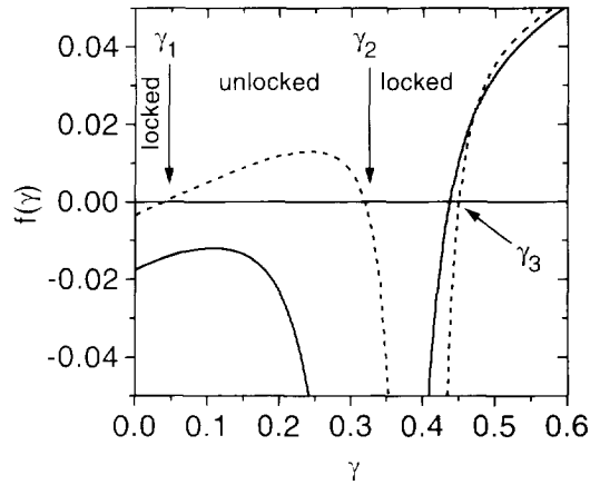
Fig. 2. Typical behavior of function f(\gamma) (12). Continuous curve: strong coupling with \Delta = 0.5 (one root), no delocking region; dashed curve: weak coupling with \Delta = 0.1 (three roots), delocking region is present. Other parameters: \alpha^A = 0.12 , \alpha^B = 0.1 , N = 3 .
