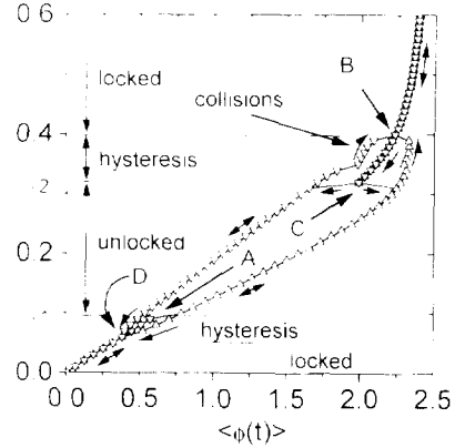
Fig. 1. I - V curve of the annular stacked JJ with delocking region. The parameters of the system are: J = 0.5 , \alpha^A/\alpha^B = 1.5 , N = 3 , L = 5 . A and C are delocking points, B and D are relocking points.
